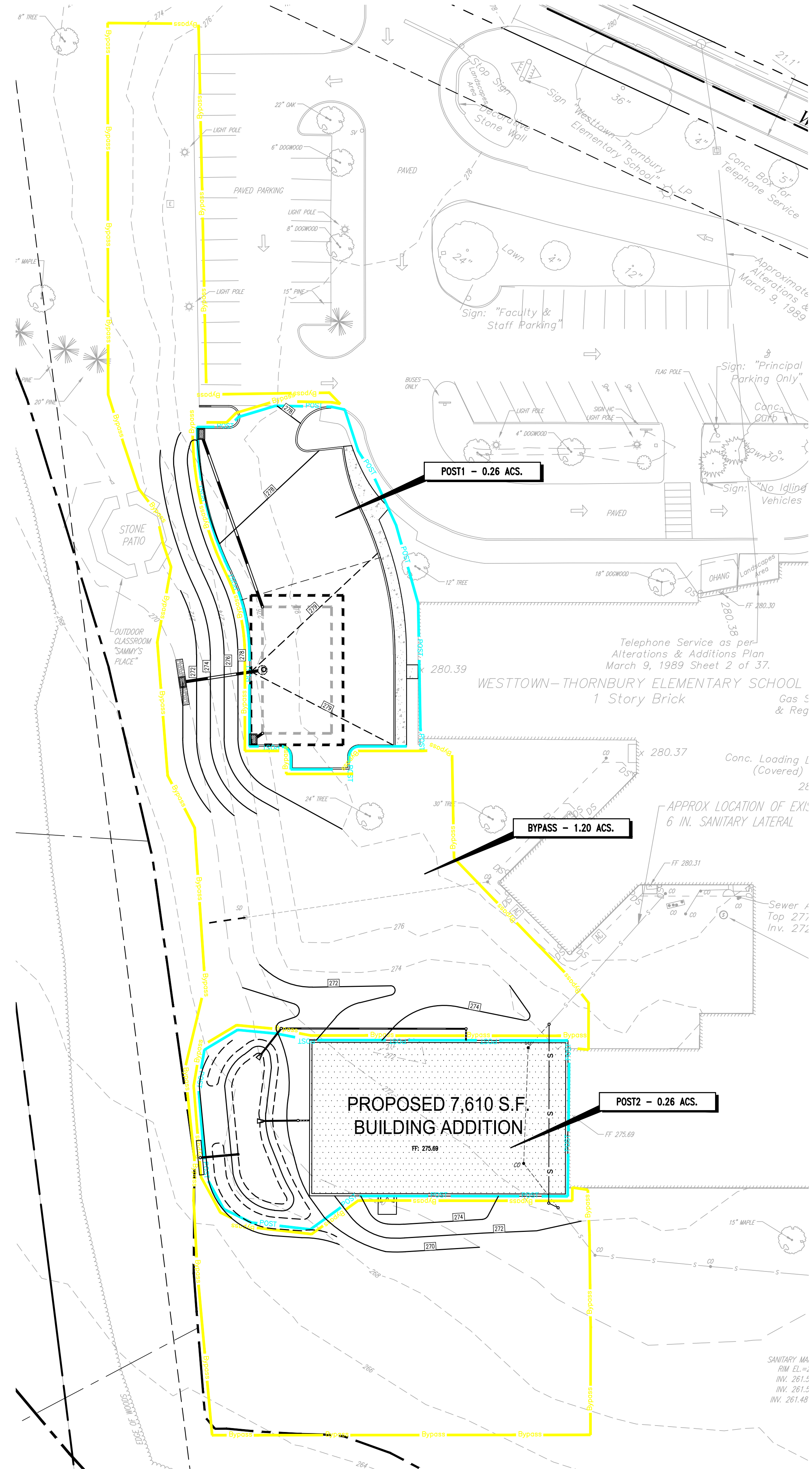
PCSM PLAN SCALE: 1" = 30'
